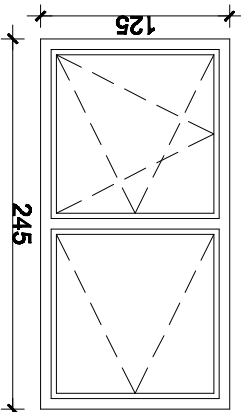
st.G/1.c-prozor vel.125x245cm
