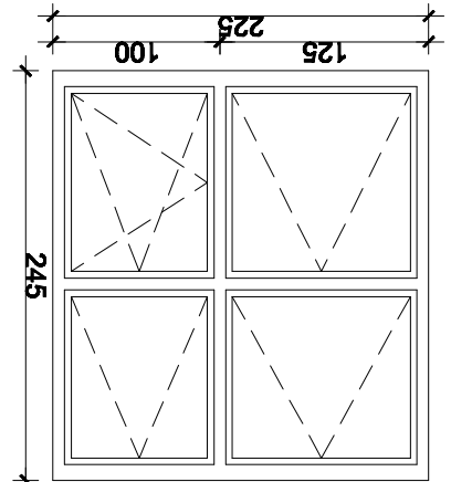
st.G/1.a-prozor vel.225x245cm
